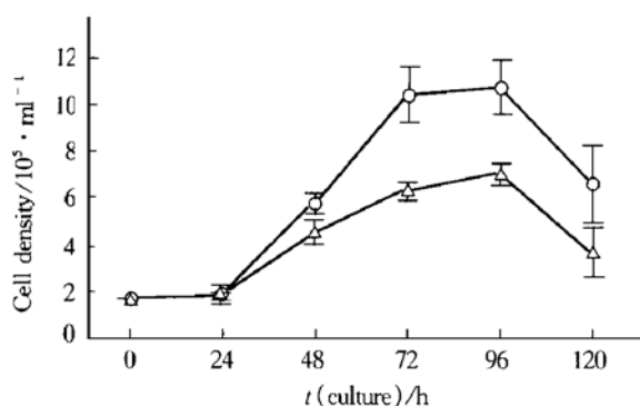
Fig. 2 Growth of hybridoma cells cultured in the medium with and without 1% gelatin
