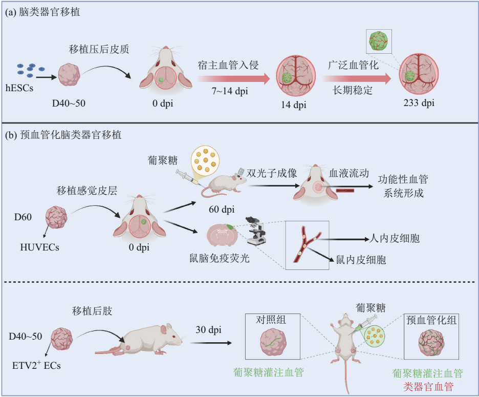
Fig. 4 Vascularization using animal host vasculature
