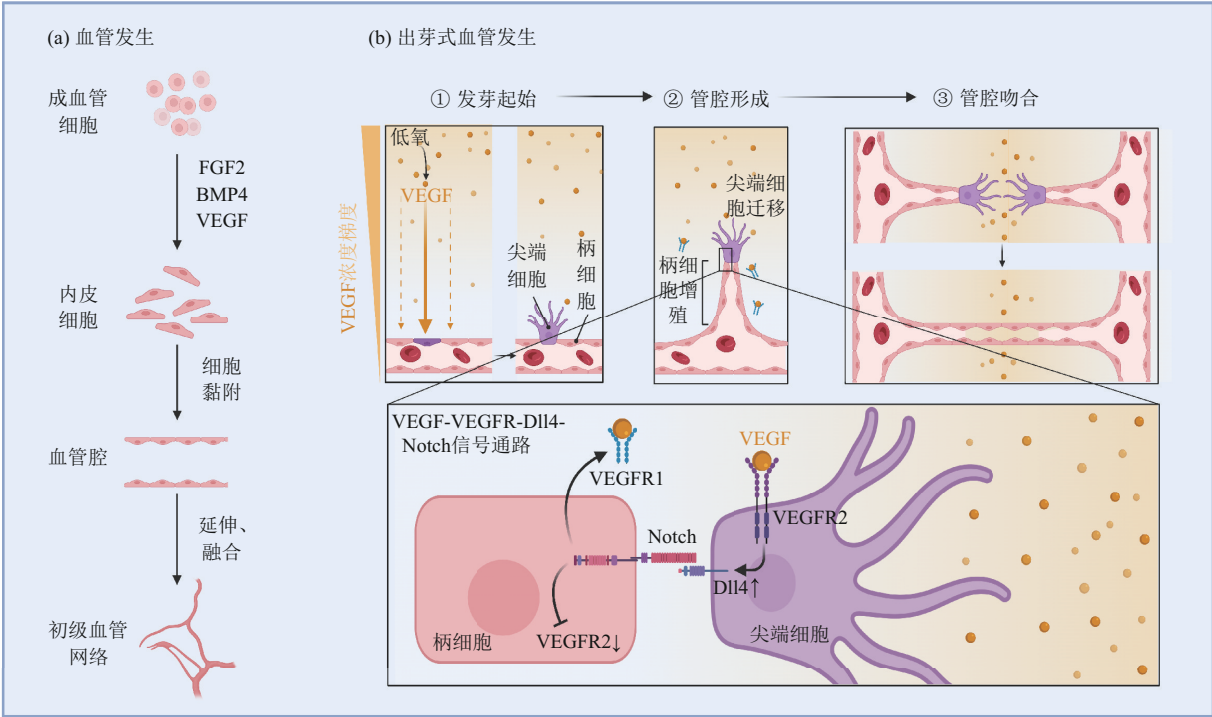
Fig. 1 Development process of cerebral vessels
