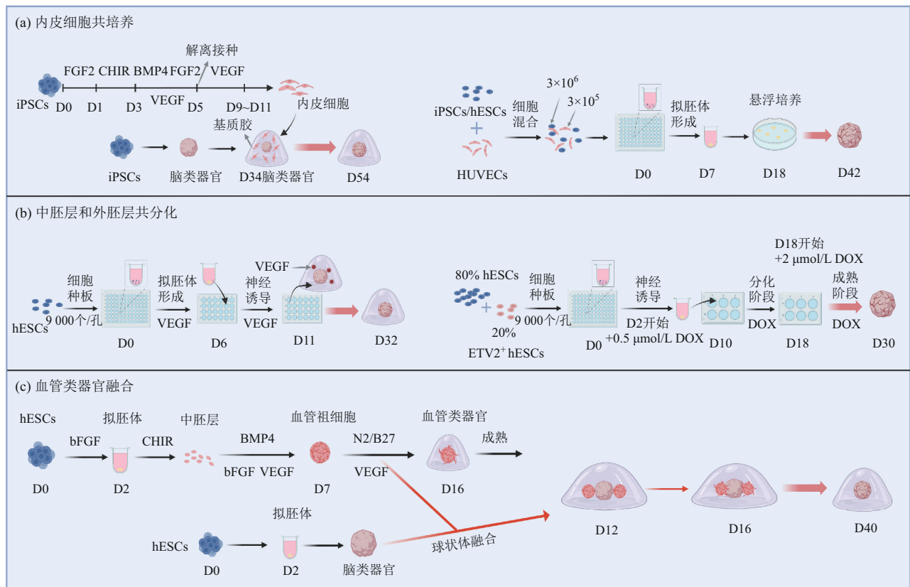
Fig. 2 Vascularization using biological self-organization methods
