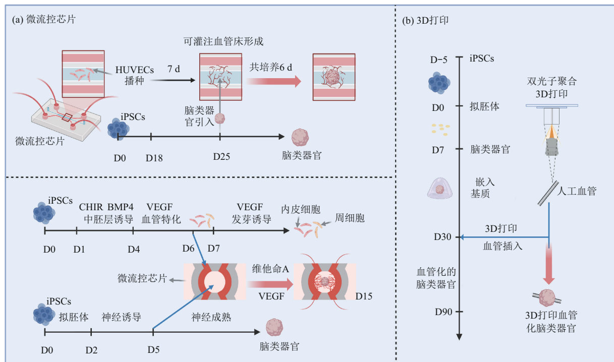
Fig. 3 Vascularization using tissue engineering strategies
