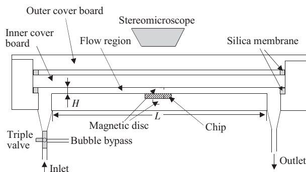
Fig.1 Schematic diagram of the flow chamber apparatus
