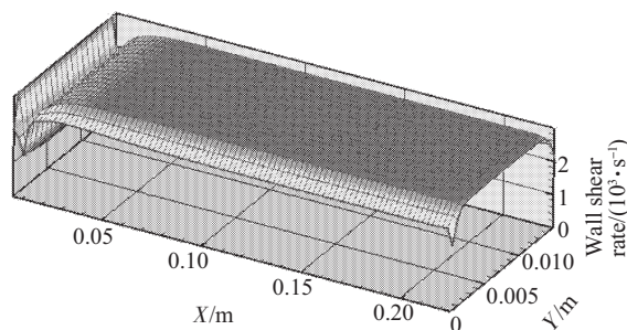
Fig.2 Numerical simulation result of wall shear rate on the chamber bottom
